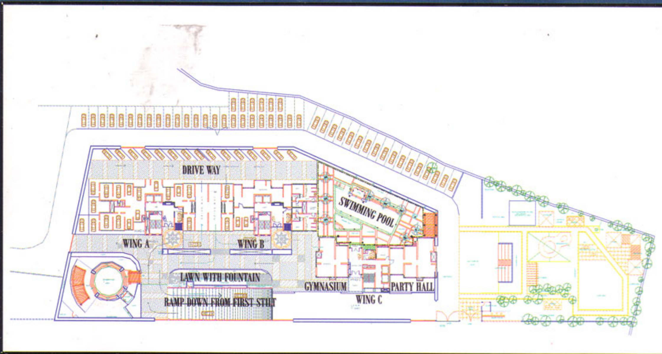
LAYOUT PLAN
